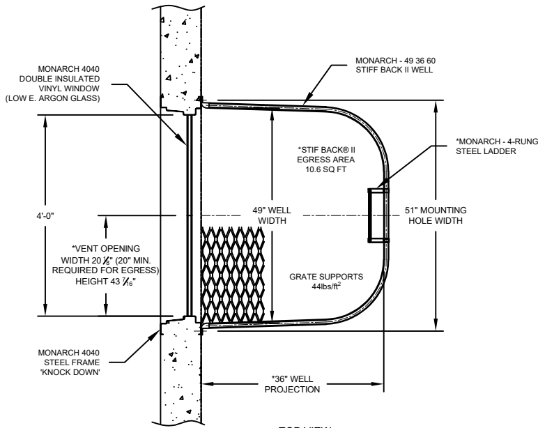
TOP VIEW WINDOW WELL
