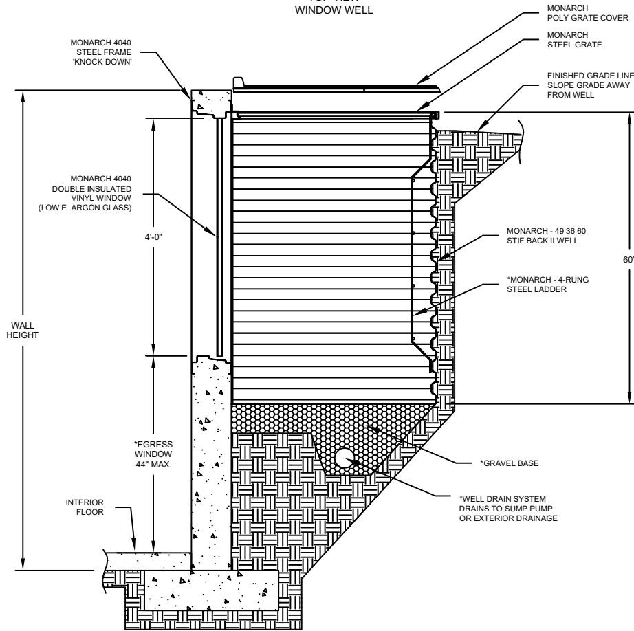
SECTION VIEW MIDLINE THRU. WINDOW AND WELL
